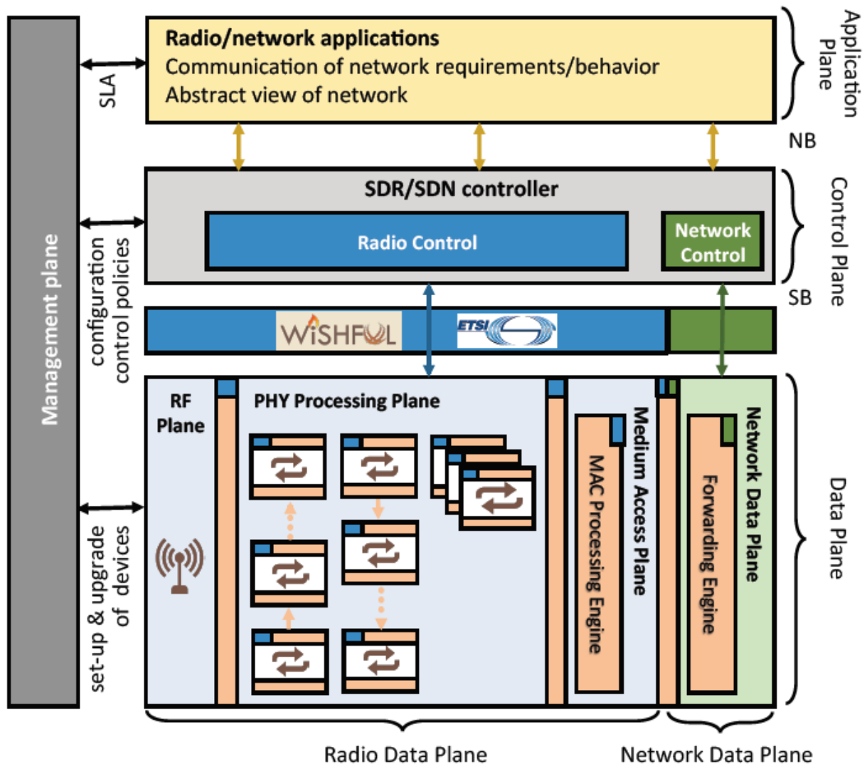
Figure 1 The ORCA architecture will focus on novel PHY and MAC functionality that can be controlled and reconfigured in real-time.
